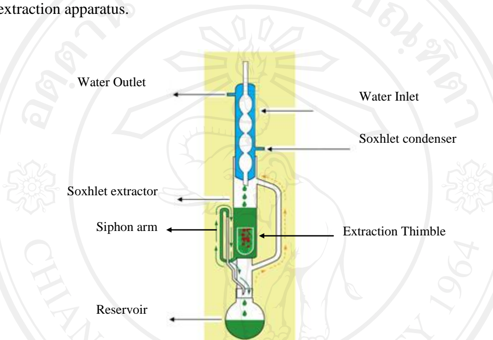
Fig. 1.11 Soxhlet extraction [4].
