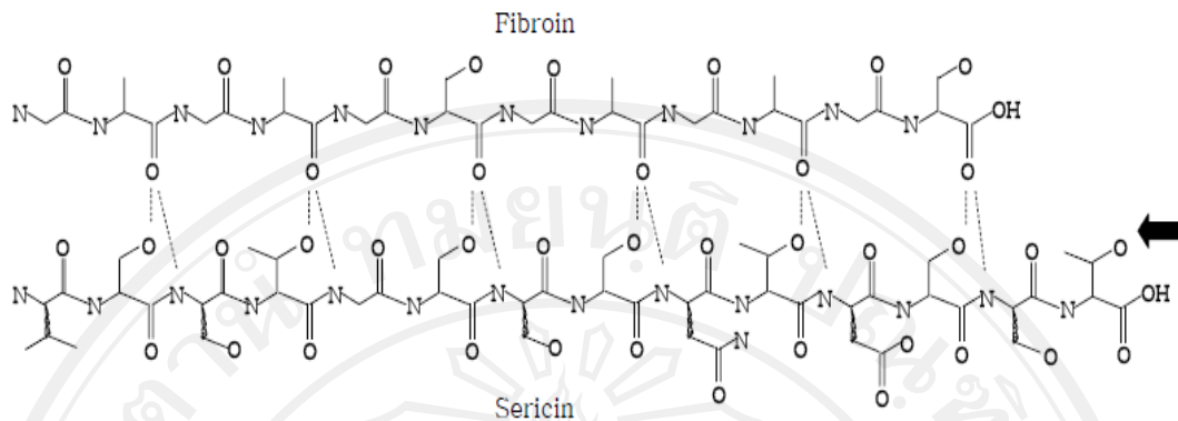
Fig. 1.33 Schematic representation of the intermolecular hydrogen bonding at the boundary of silk fibroin and silk sericin [101].
