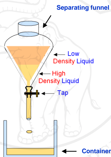
Fig. 1.9 Funnel separation [13].
