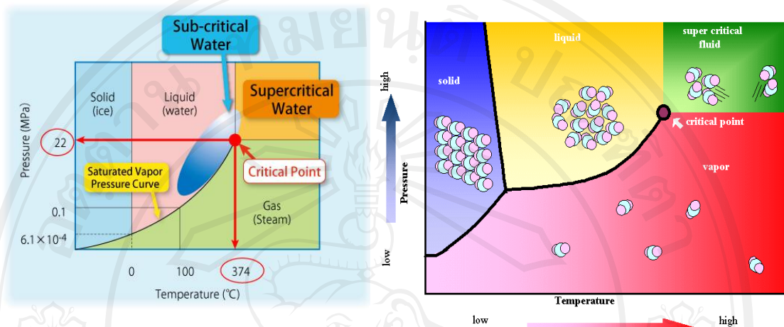
Fig. 1.14 The phase diagram of water [22].
