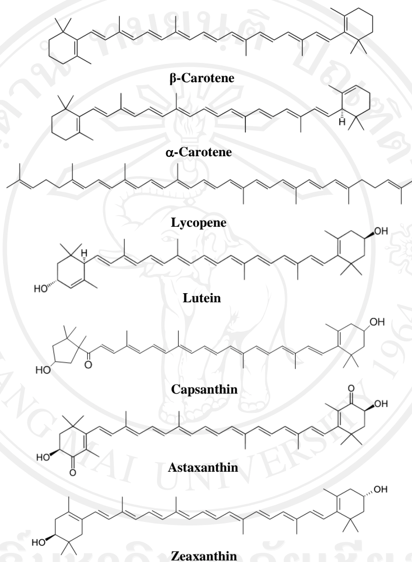
Fig. 1.27 Chemical structure of some carotenoids [70].
