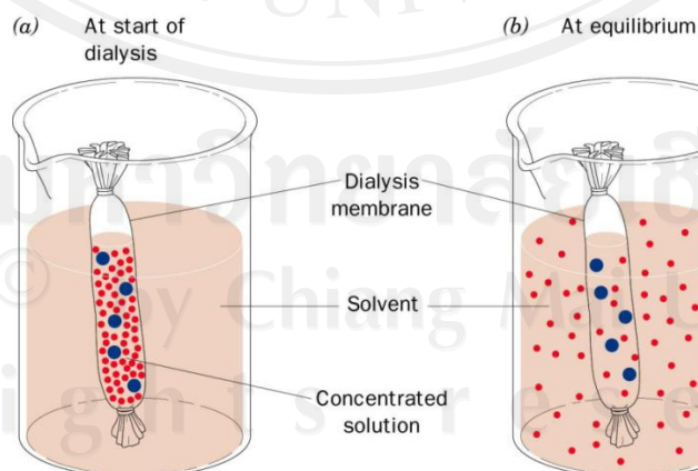
Fig. 1.16 Dialysis [26].
