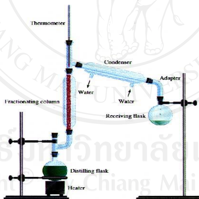
Fig. 1.8 Fractional distillation [12].
