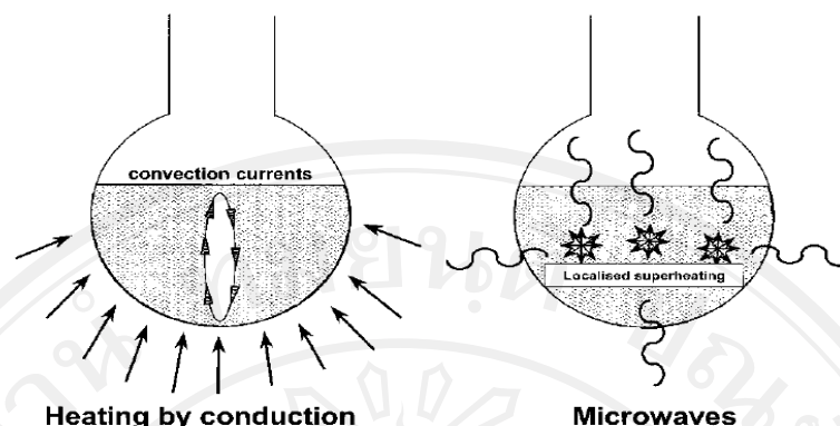
Fig. 1.13 The heating principles of classical conduction and the MAE [21].
