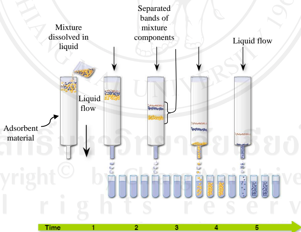
Fig. 1.7 Column chromatography [11].
