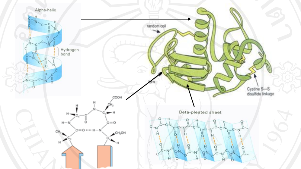
Fig. 1.32 Secondary structure of proteins include random coil (no structure), alpha-helix , the beta-sheet , and the turn [99, 100].
