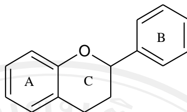
Fig. 1.29 Basic flavonoid structure [67].
