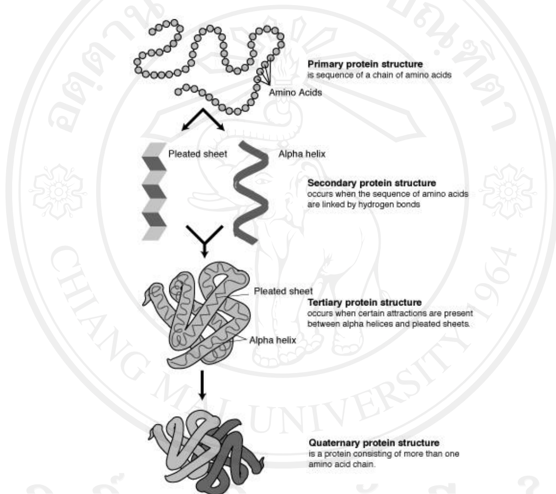
Fig. 1.31 Common structure of protein [98].
