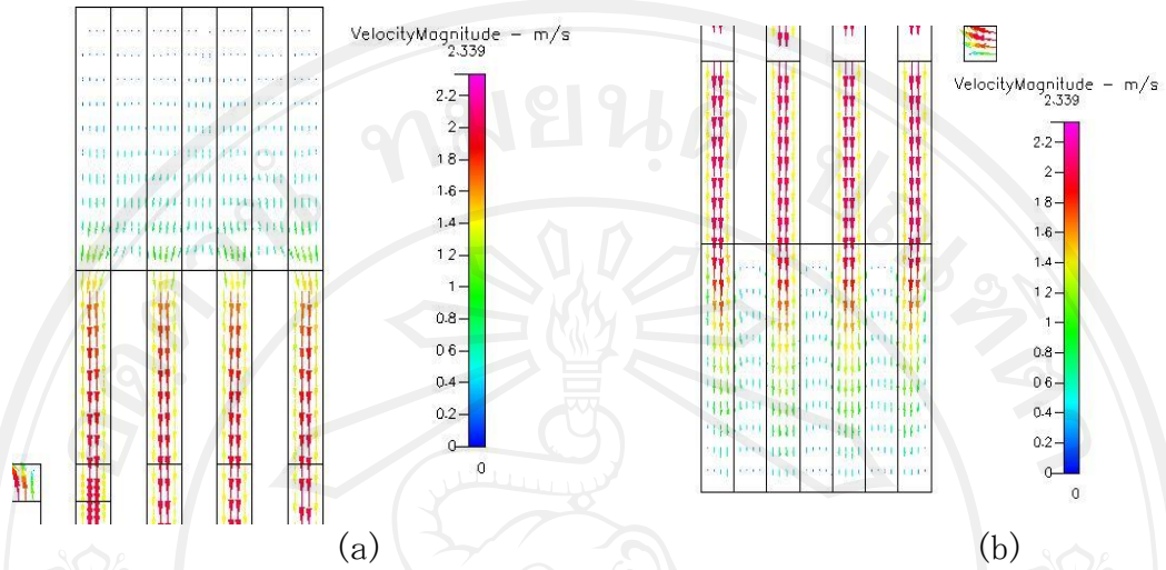
Figure 5.60 Characteristic of flow at 300 \text{ cm}^3/\text{min} in manifold 4 channels
