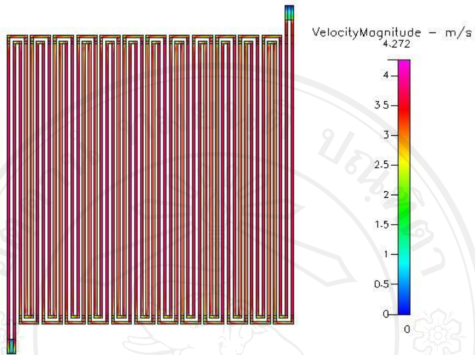
Figure 5.48 Velocity distribution at 300 \text{ cm}^3/\text{min} of manifold 2 channels
