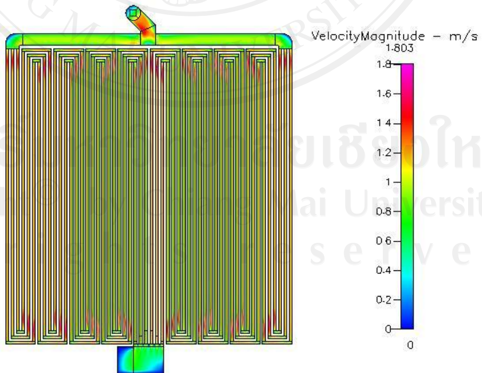
Figure. 5.83 2 ways multi-serpentine header flow field
