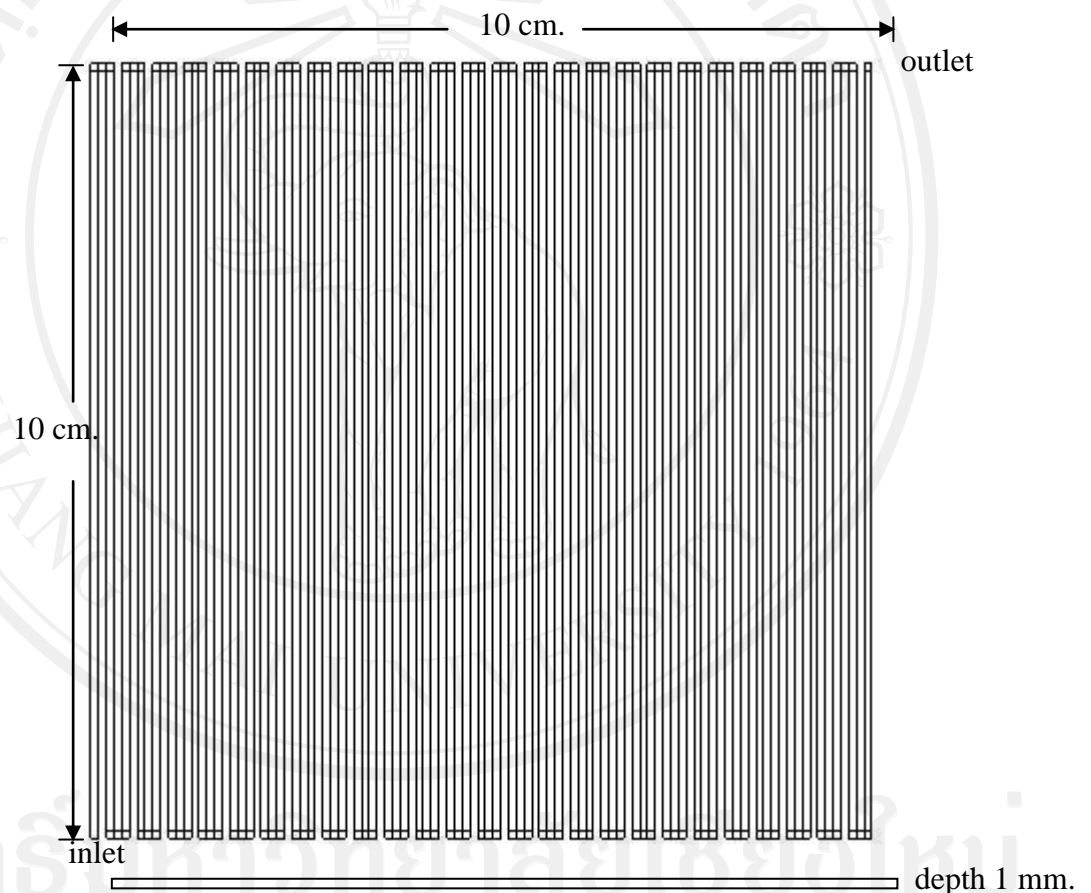
Figure 5.2 Serpentine flow filed pattern modeling
