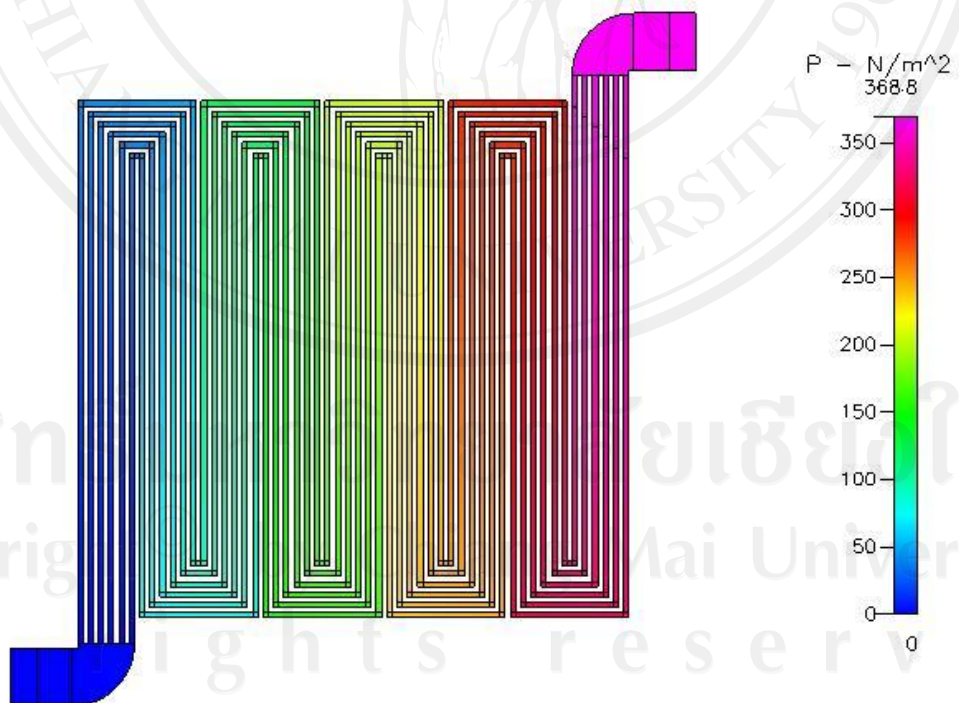
Figure 5.70 Pressure distribution at 300 \text{ cm}^3/\text{min} of type 2 manifold
