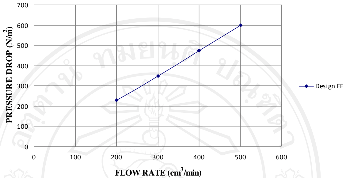
Figure 5.89 Pressure drop and flow rate
