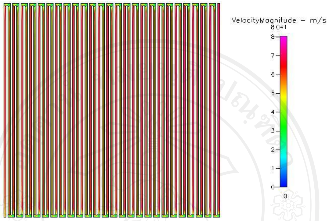
Figure 5.5 Velocity distribution at 300 \text{ cm}^3/\text{min} of inside fillet curve
