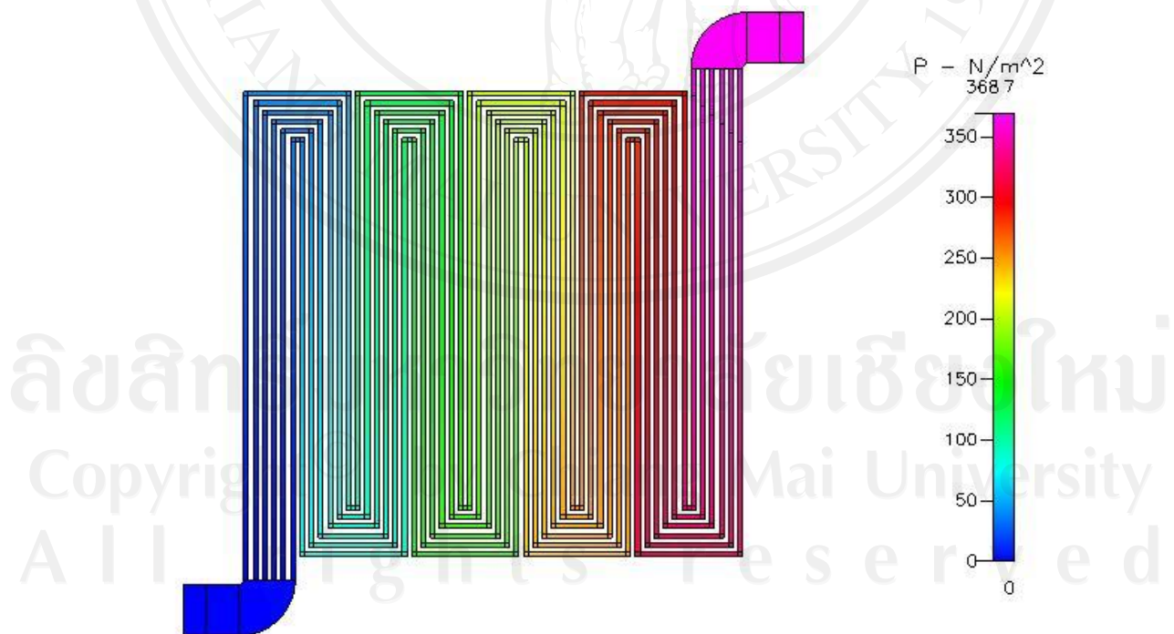
Figure 5.72 Pressure distribution at 300 \text{ cm}^3/\text{min} of type 3 manifold
