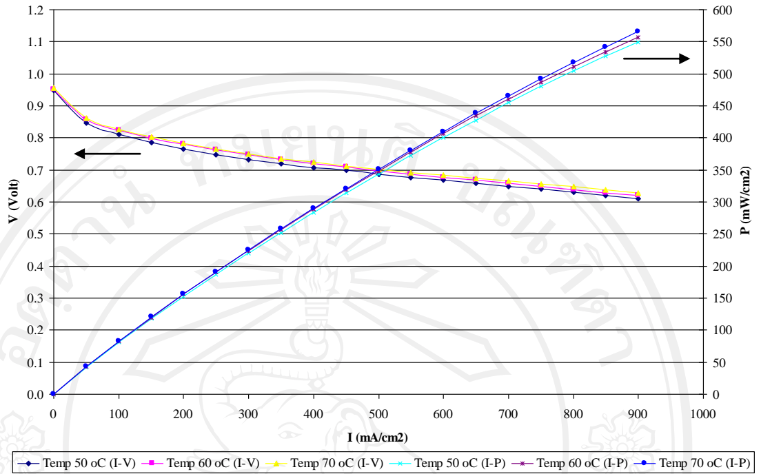
Figure 5.102 Performance curve of 4 serpentine channels fuel cell
