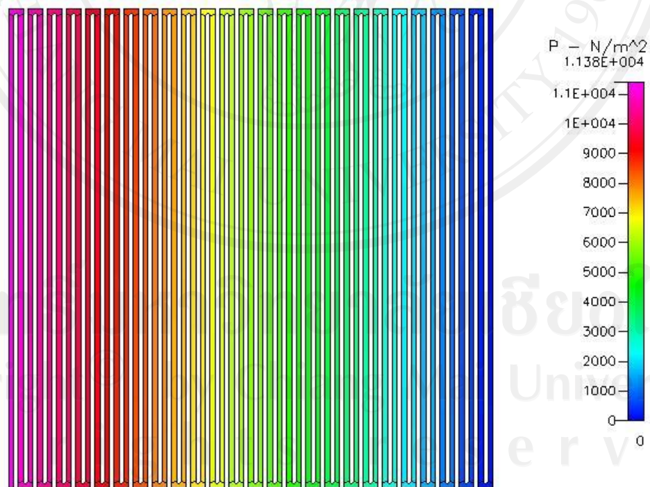
Figure 5.6 Pressure distribution at 300 \text{ cm}^3/\text{min} of inside fillet curve
