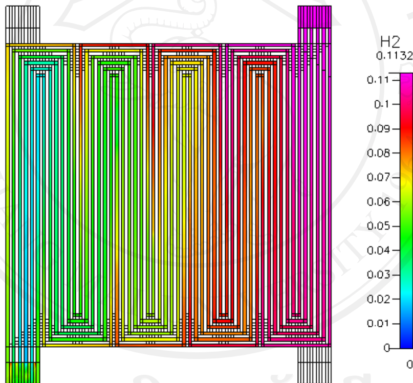
Figure 5.91 \text{H}_2 in anode at 500 \text{cm}^3/\text{min} of 6 serpentine channels
