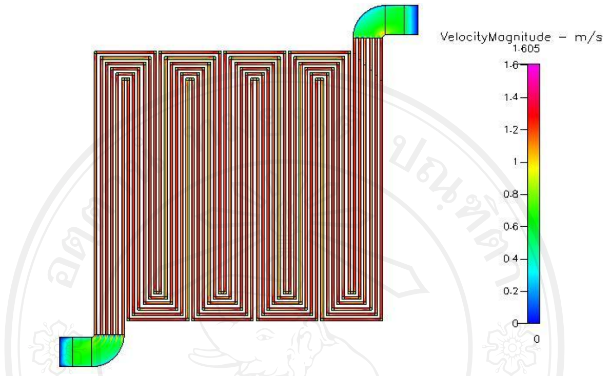
Figure 5.71 Velocity distribution at 300 \text{ cm}^3/\text{min} of type 3 manifold
