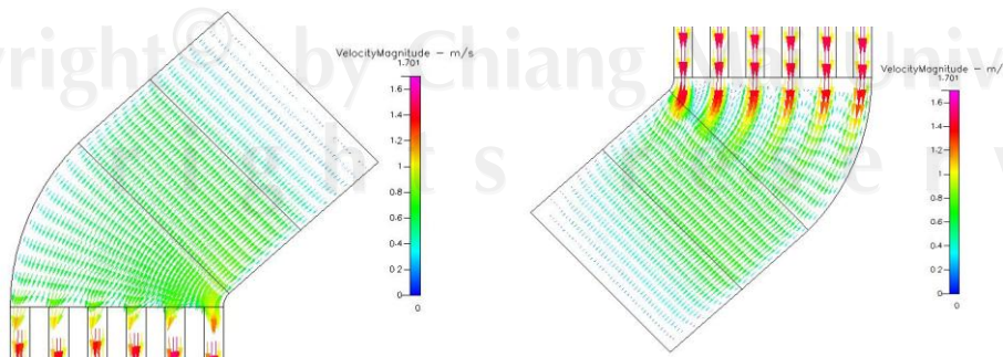
Figure 5.78 Characteristic of flow at 300 \text{ cm}^3/\text{min} in type 4 channels
