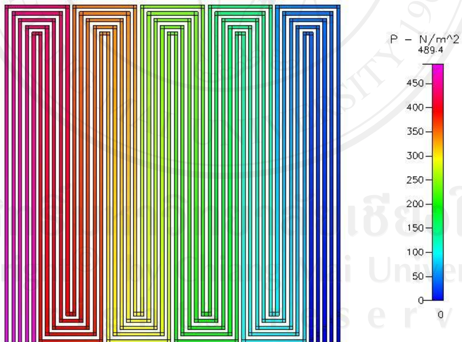
Figure 5.27 Pressure distribution at 300 \text{ cm}^3/\text{min} of 5 channels
