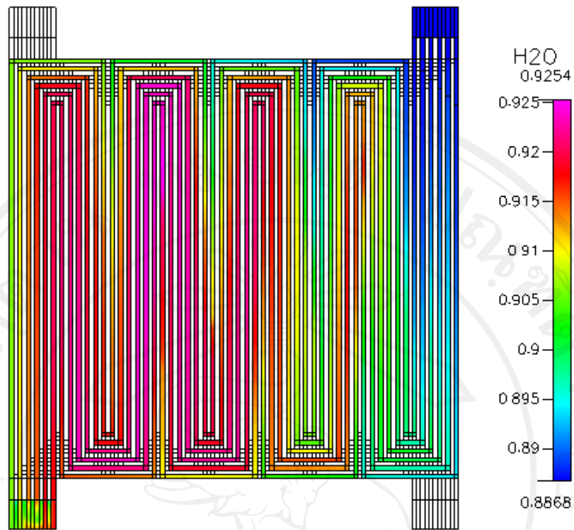
Figure 5.92 H 2 O in anode at 500 cm 3 /min of 6 serpentine channels
