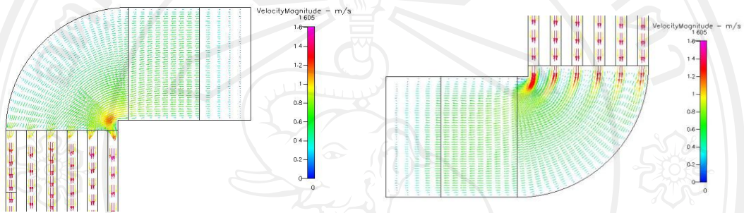
Figure 5.76 Characteristic of flow at 300 \text{ cm}^3/\text{min} in type 2 manifold (a) inlet (b) outlet
