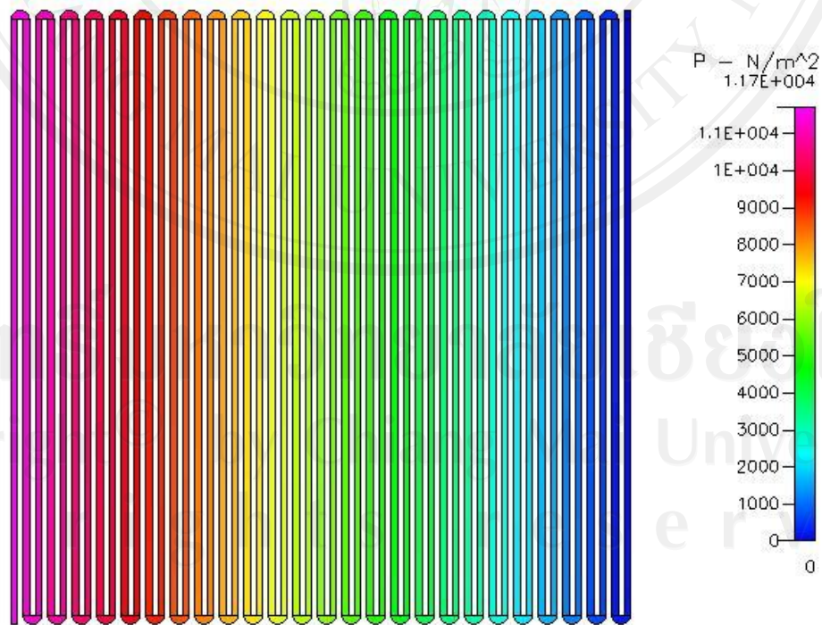
Figure 5.8 Pressure distribution at 300 \text{ cm}^3/\text{min} of outside fillet curve
