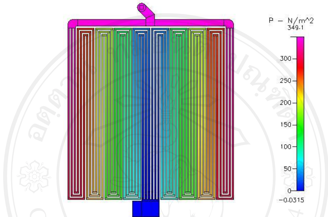
Figure 5.85 Pressure distributions at 300 \text{ cm}^3/\text{min} of first design flow field
