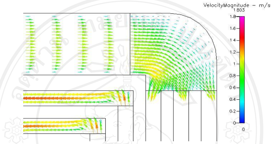
Figure 5.87 Curve velocity distribution at 300 \text{ cm}^3/\text{min} of first design flow field
