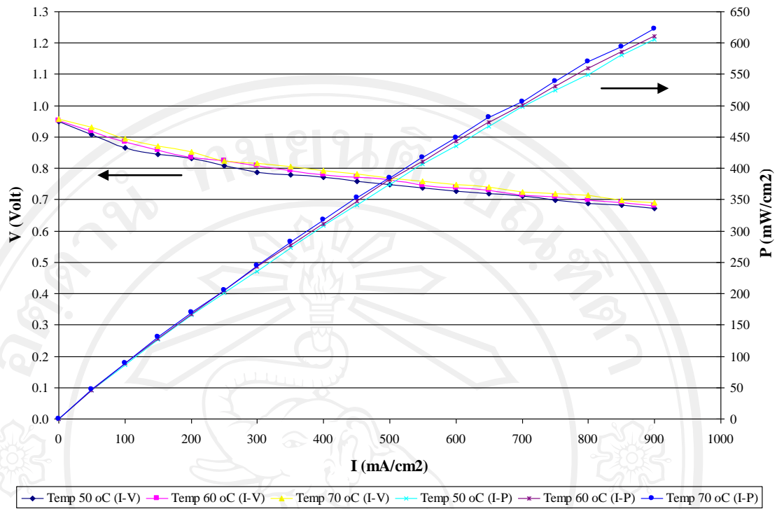
Figure 5.104 Performance curve of 2 ways multi-serpentine channels fuel cell
