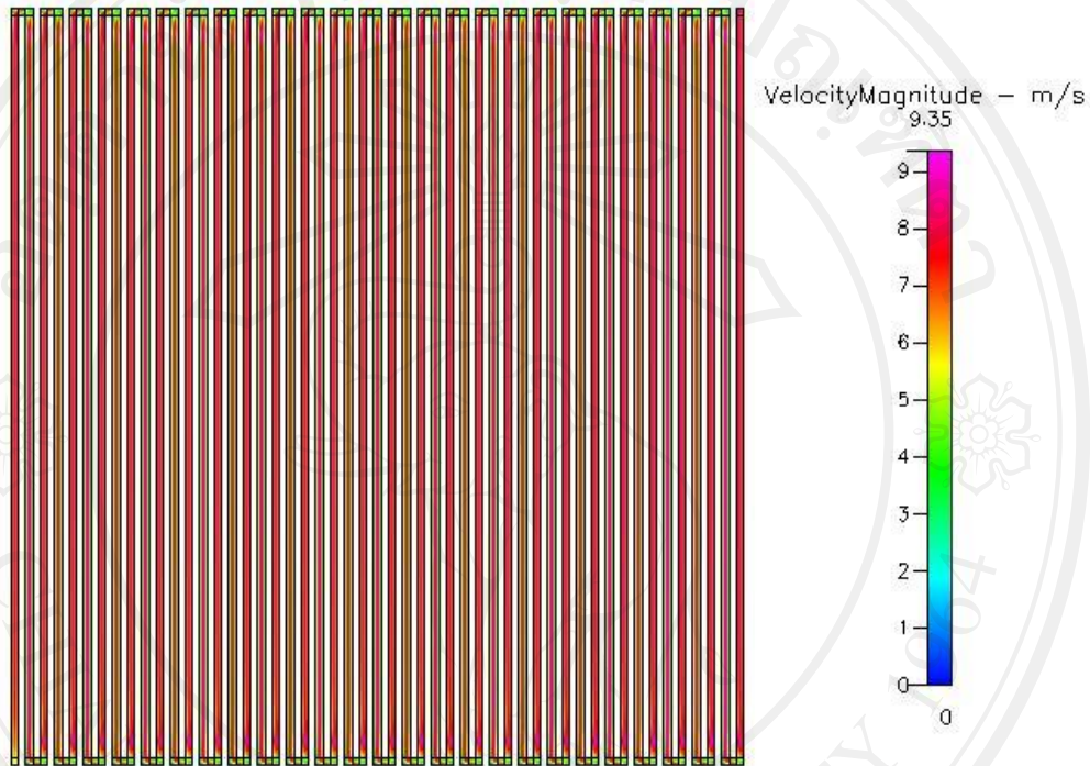
Figure 5.33 Velocity distribution at 300 cm 3 /min of 0.8 mm. depth
