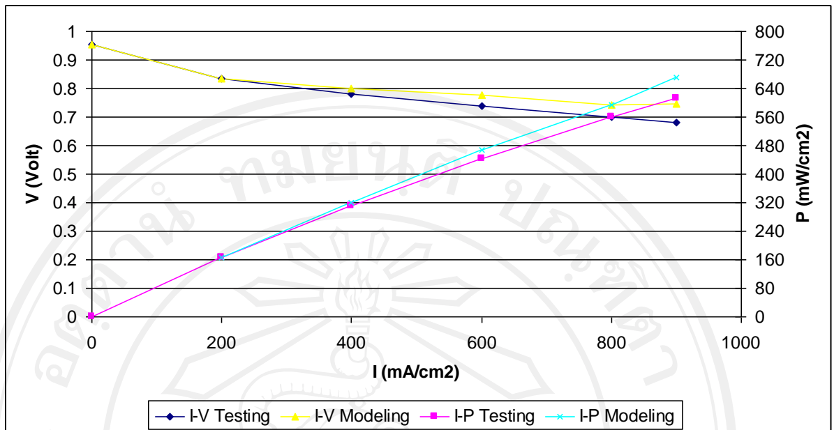
Figure 5.101 Comparison of model and experimental polarization curves.
