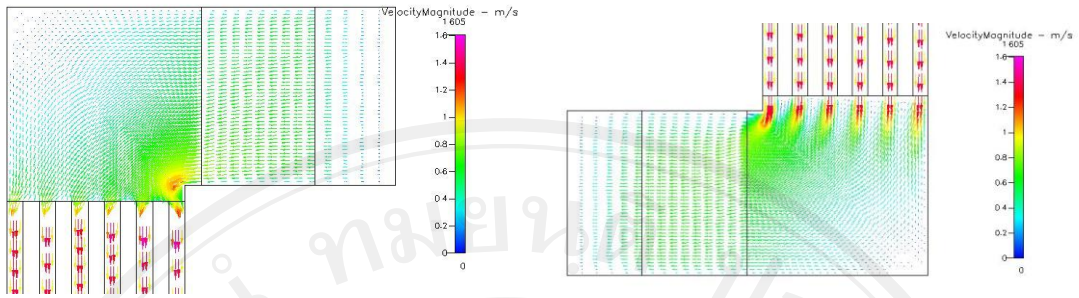
Figure 5.75 Characteristic of flow at 300 \text{ cm}^3/\text{min} in type 1 manifold (a) inlet (b) outlet
