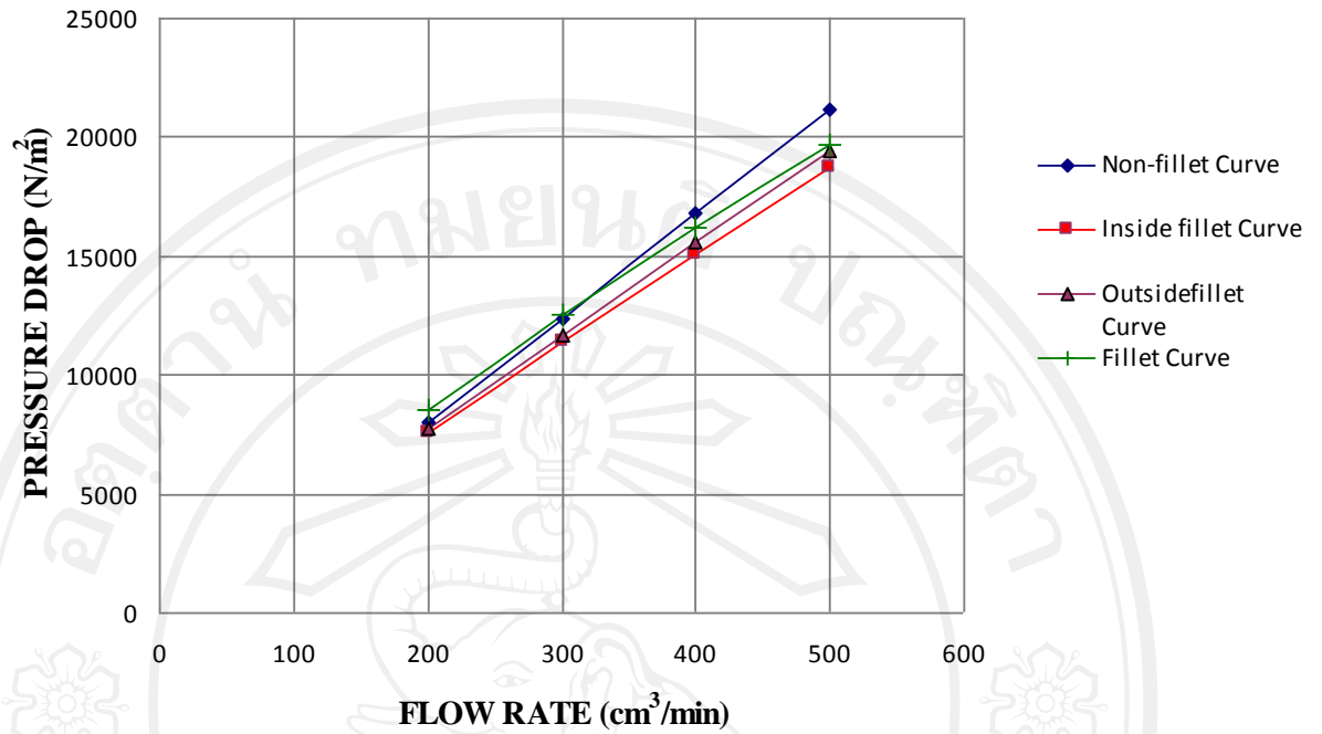
Figure 5.17 Pressure drop and flow rate in different channel curve
