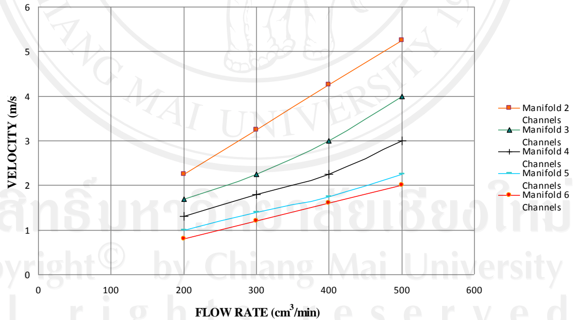
Figure 5.64 Velocity at depth 0.5 mm. and flow rate in different manifold pattern
