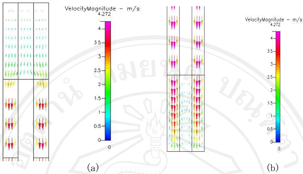
Figure 5.58 Characteristic of flow at 300 \text{ cm}^3/\text{min} in manifold 2 channels
