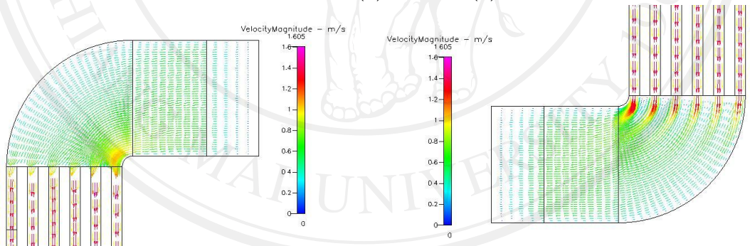
Figure 5.76 Characteristic of flow at 300 \text{ cm}^3/\text{min} in type 2 manifold (a) inlet (b) outlet
