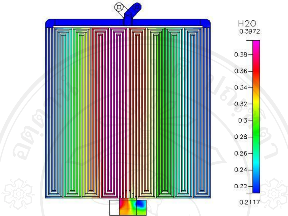
Figure 5.99 H 2 O in cathode at 500 cm 3 /min of 2 ways multi-serpentine with header flow field
