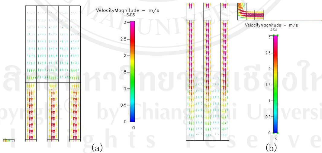
Figure 5.59 Characteristic of flow at 300 \text{ cm}^3/\text{min} in manifold 3 channels
