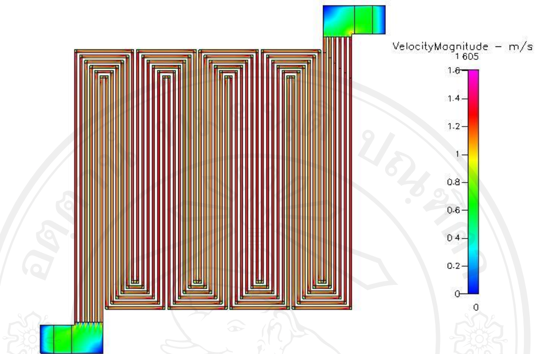
Figure 5.67 Velocity distribution at 300 \text{ cm}^3/\text{min} of type 1 manifold
