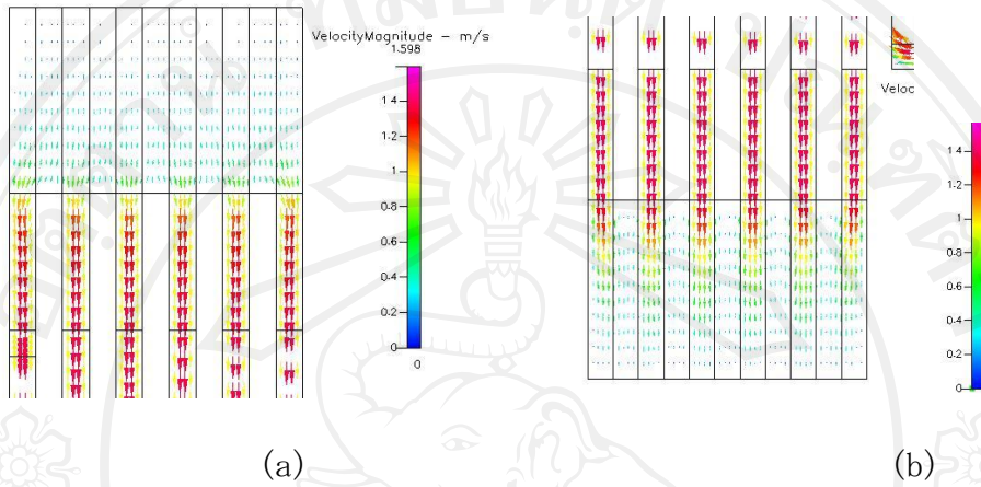
Figure 5.62 Characteristic of flow at 300 \text{ cm}^3/\text{min} in manifold 6 channels
