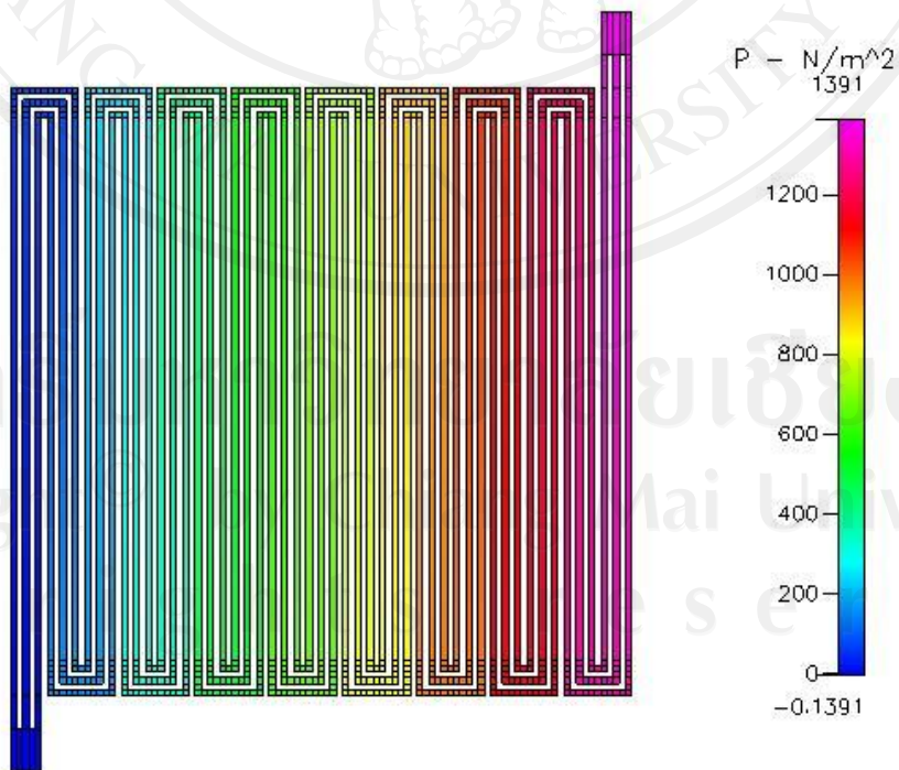
Figure 5.51 Pressure distribution at 300 \text{ cm}^3/\text{min} of manifold 3 channels
