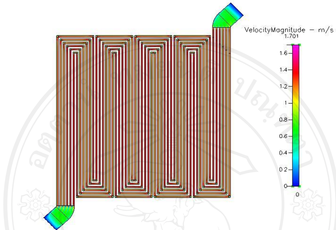
Figure 5.73 velocity distribution at 300 \text{ cm}^3/\text{min} of type 4 manifold
