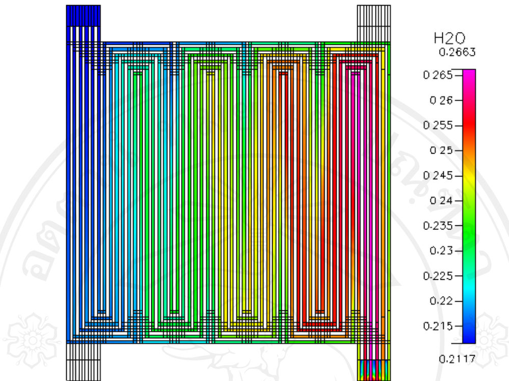
Figure 5.94 H 2 O in cathode at 500 cm 3 /min of 6 serpentine channels
