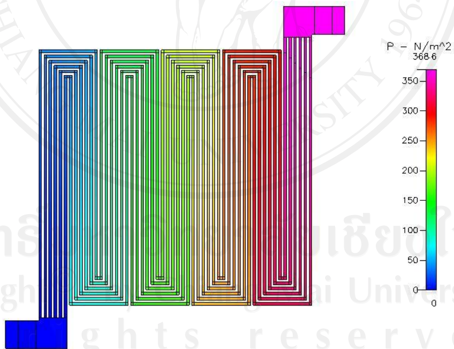
Figure 5.68 Pressure distribution at 300 \text{ cm}^3/\text{min} of type 1 manifold
