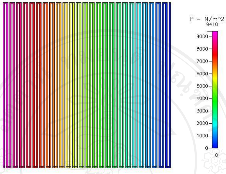
Figure 5.36 Pressure distribution at 300 cm 3 /min of 1.2 mm. depth
