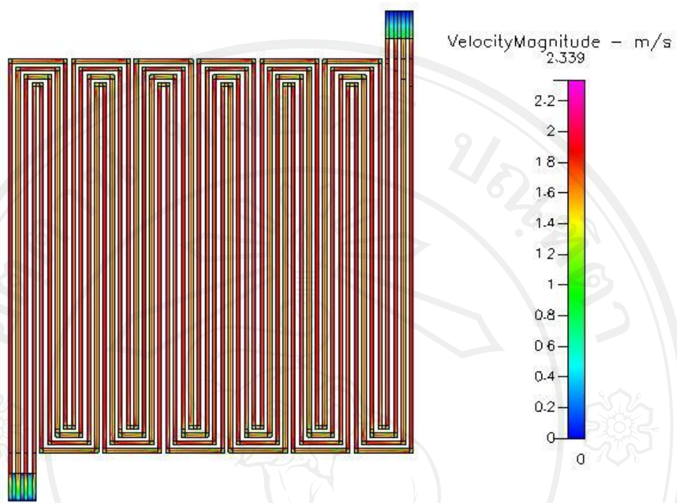
Figure 5.52 Velocity distribution at 300 \text{ cm}^3/\text{min} of manifold 4 channels
