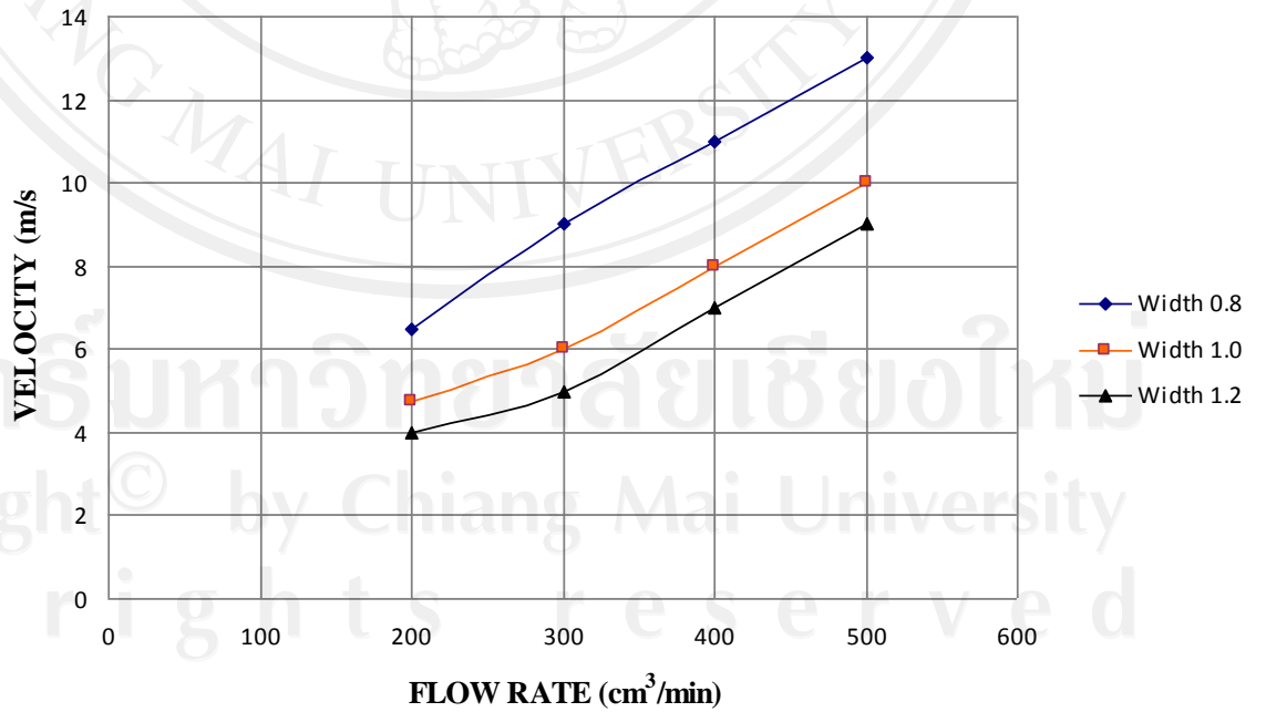
Figure 5.45 Velocity at depth 0.5 mm and flow rate in different channel width
