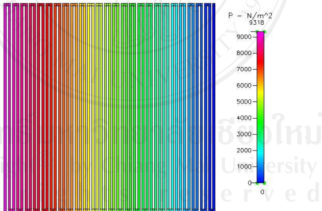
Figure 5.43 Pressure distribution at 300 \text{ cm}^3/\text{min} of 1.2 mm. width
