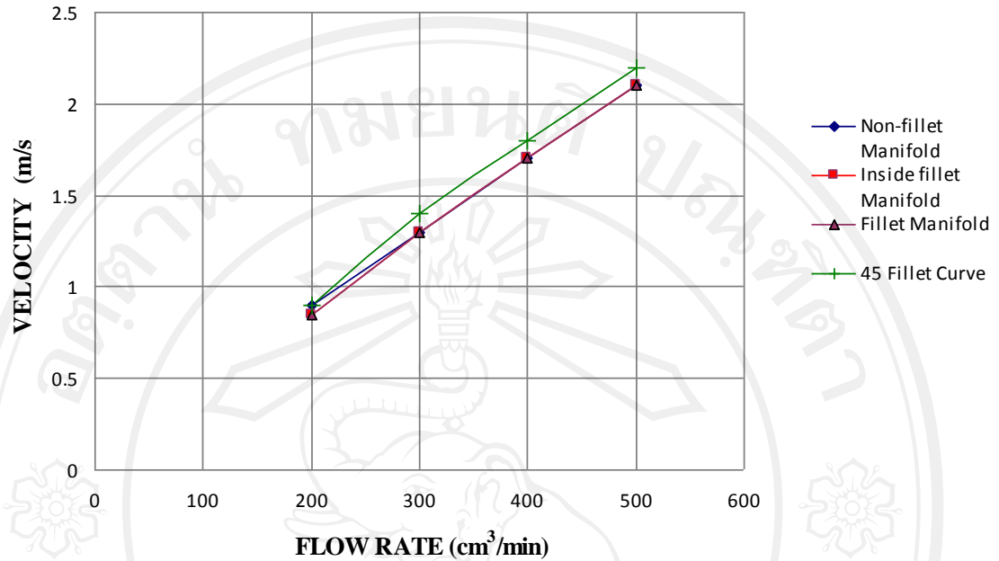
Figure 5.81 Velocity at depth 0.5 mm. and flow rate in different manifold pattern
