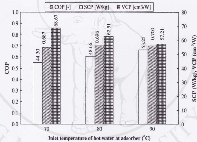
Fig. 4. Relationship of COP, SCP, and VCP with the heat source temperature without the sound wave
