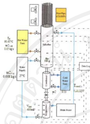
Fig. 3 Experimental set up for the CLOHP test
