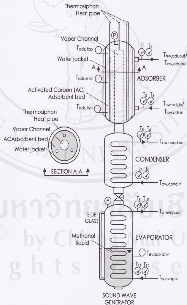
Fig. 2. Schematic sketches of the experiment apparatus
