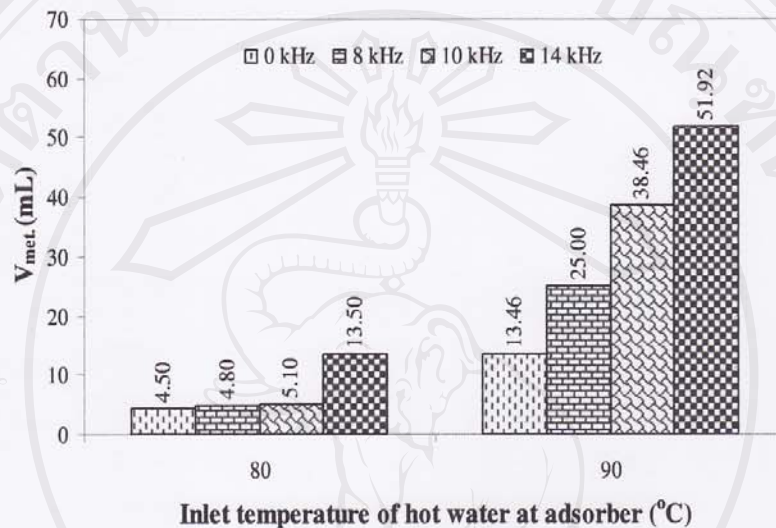
Figure 3. Effect of the hot water temperature at the inlet of the adsorber on the volume of methanol condensate.
