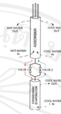
Fig. 4 Experimental set up of the control valve test
