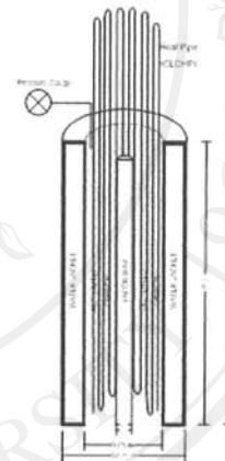
Fig. 2 Closed-loop oscillating heat pipe in adsorber
