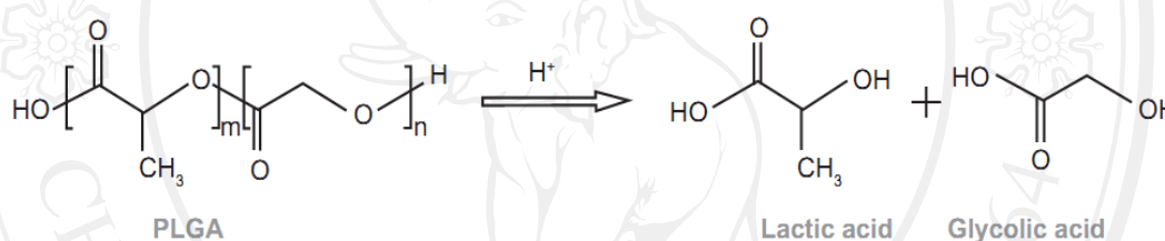
Figure 8: Hydrolysis of PLGA nanoparticles (44)
