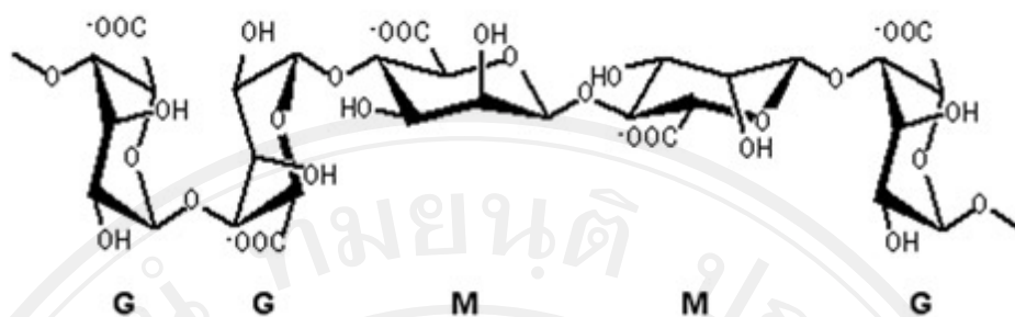
Figure 6: The structure of chain conformation of alginate (43)
