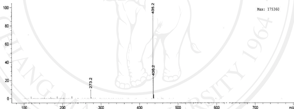
Figure 41: Mass spectrum of ethanolic crude extract at 44.371 min
