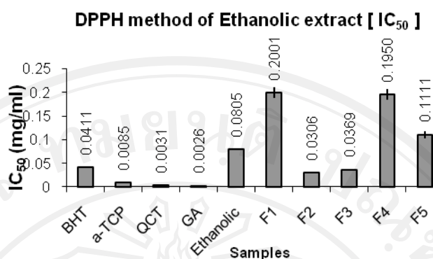
Figure 33: Free radical-scavenging activity of B. monosperma flowers extracts were expressed as IC 50 value, EtOAc extract (A), and Ethanolic extract (B) by DPPH method
