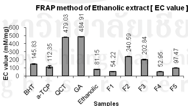
Figure 32: Reducing power of B. monosperma flowers extracts were expressed as EC value, EtOAc extract (A), and Ethanolic extract (B) by FRAP method
