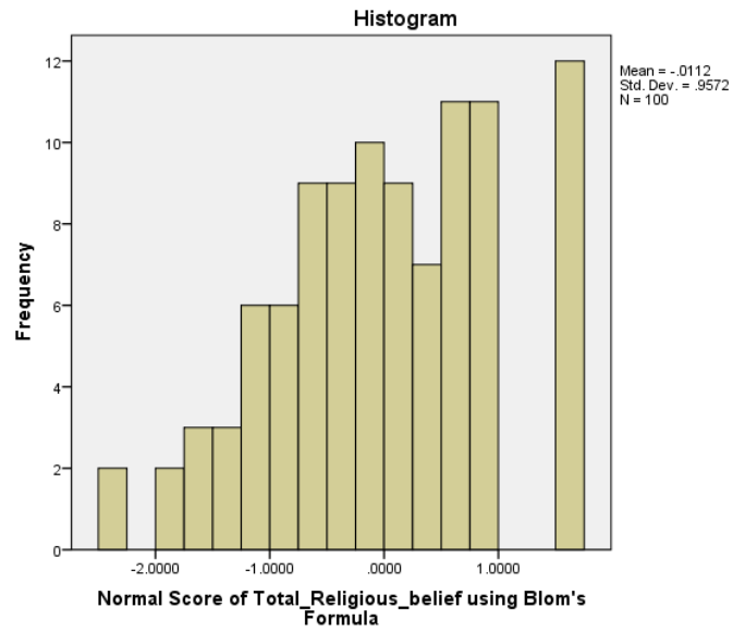
Figure H-1 Histogram of the Study Variables
