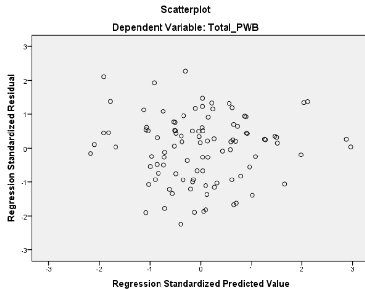
Figure H-2 The scatter Plots of the Standardized Residuals by the Regression Standardized Predicted Value
